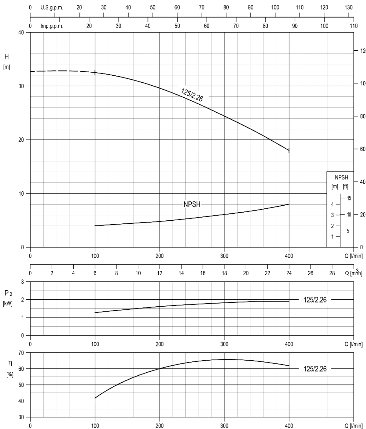
32-125/2.26 (2.2kW) – Impeller diameter = 133 mm
